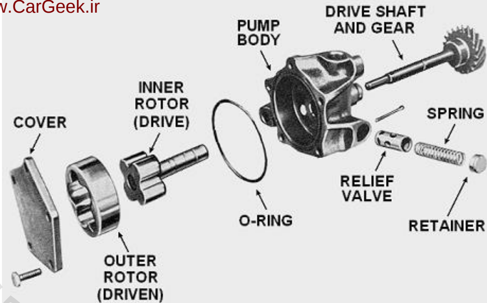
Rotor type pump
